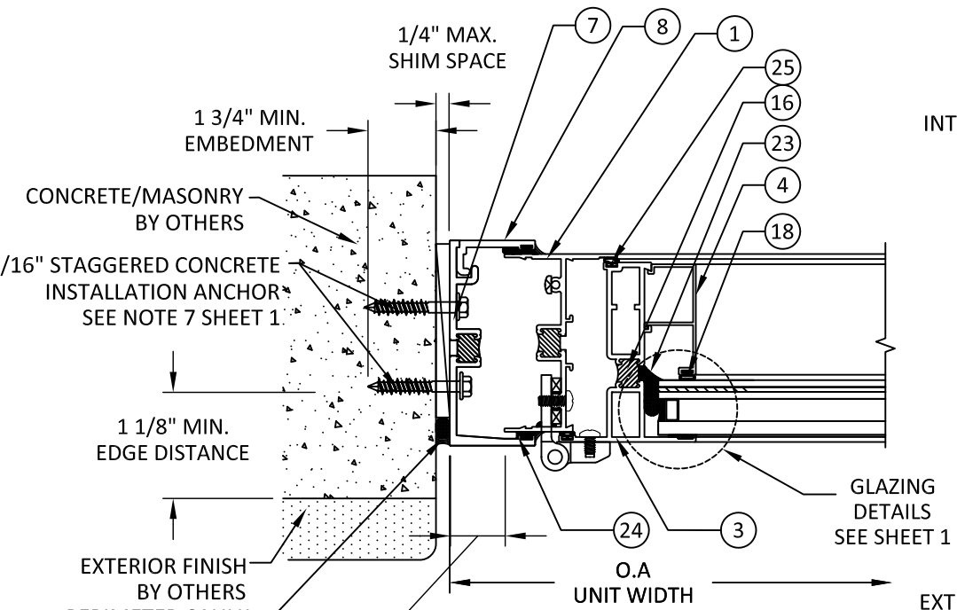
G HORIZONTAL SECTION 5 JAMB - CONCRETE OR CMU THROUGH FRAME INSTALLATION
