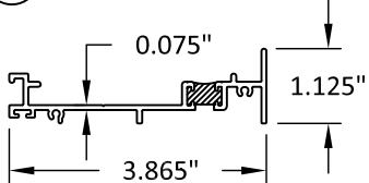
⑨ 3 1/4" SUBSILL
