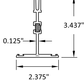
⑭ MULLION SNAP CLIP
