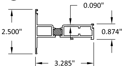
③ PROJECTED VENT FRAME
