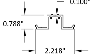
⑬ HEAVY MULLION PRESSURE CLIP
