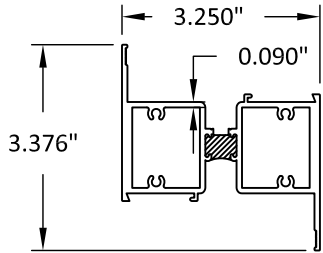
② HEAVY DUTY MTG RAIL
