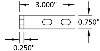
③1 T-MULLION ANCHOR BRACKET
