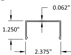
⑮ MULLION PRESSURE CLIP
