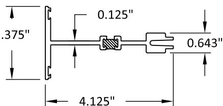
⑩ HEAVY T-MULLION
