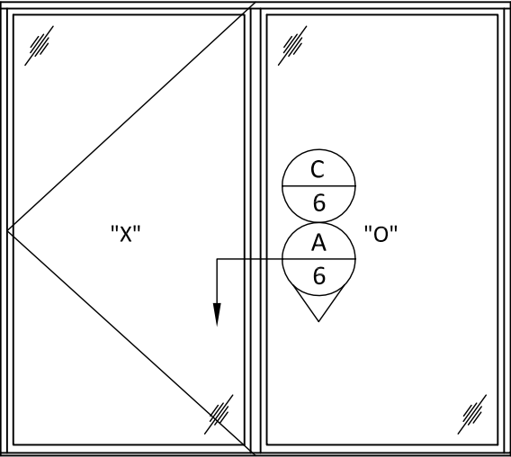
CASEMENT FIXED
