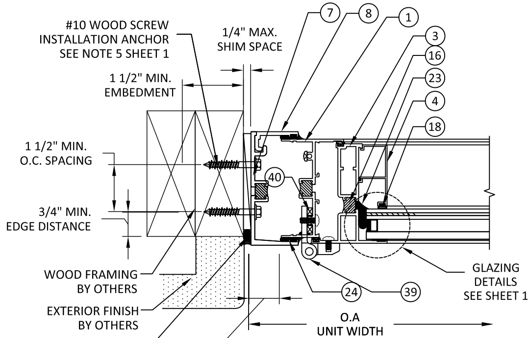
E HORIZONTAL SECTION 5 JAMB - 2X WOOD FRAME THROUGH FRAME INSTALLATION
